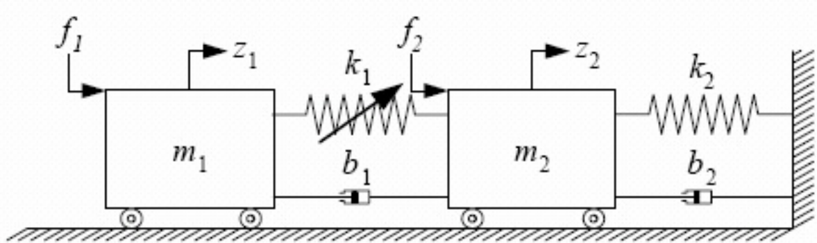
Fig. 1. Mass-spring system.
